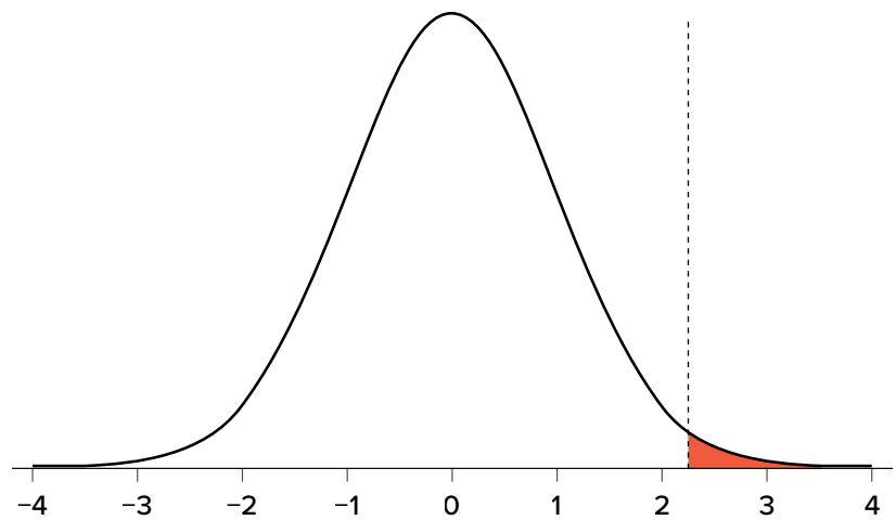
Shaded p value for z_{\text{obt}} = 2.25 ; reject H_0
